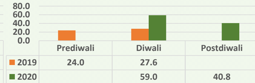
Rambagh (NO 2 )
