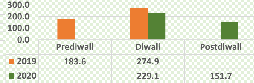
Rambagh (PM10)
